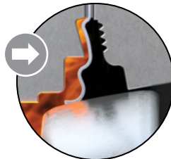
Disc in Closed Position. During and after fire. Resilient seat destroyed. Line pressure applied from preferred flow direction.
