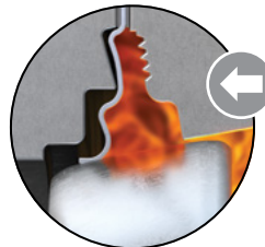
Disc in Closed Position. During and after fire. Resilient seat destroyed. Line pressure applied from non-preferred flow direction.
