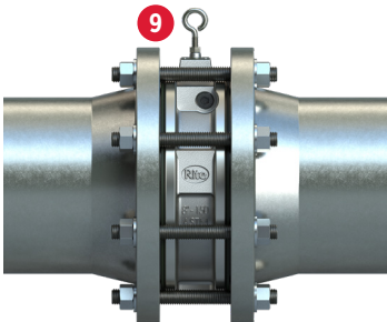
Figure 04: Integral Hard Seat In-Pipe View.
