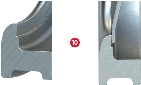
Figure 05: Integral Hard Seat Close-Up Cutaway Views.
