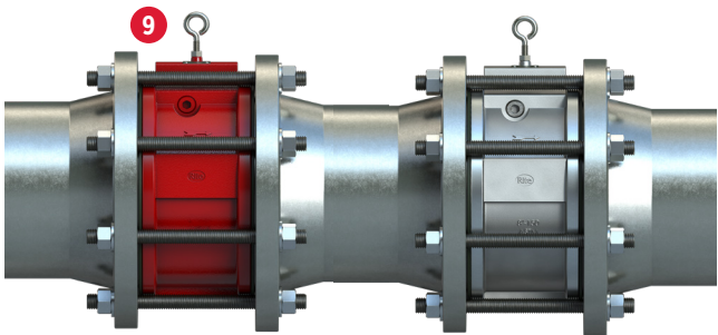
Figure 05: Integral Soft Seat Seat In-Pipe View.
