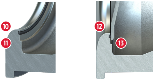
Figure 06: Integral Soft Seat Close-Up Cutaway Views.
