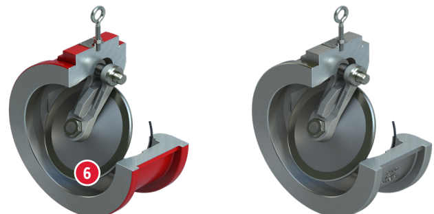
Figure 02: Integral Soft Seat Cutaway Rear View.
