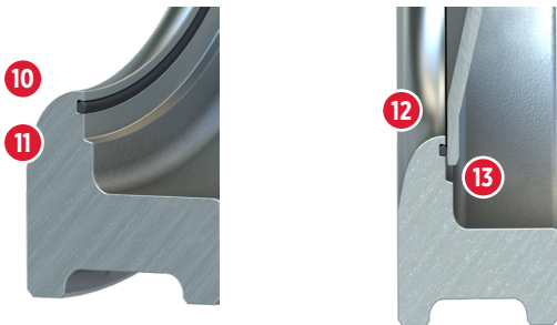
Figure 06: Integral Soft Seat Close-Up Cutaway Views.
