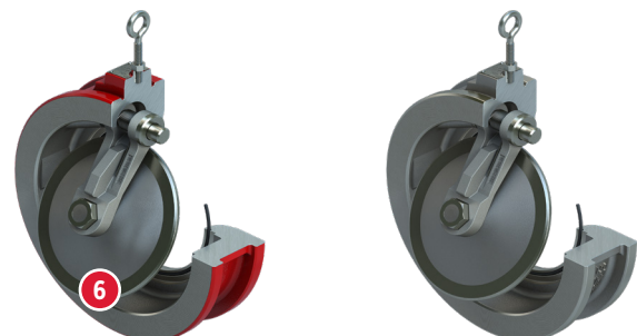
Figure 02: Integral Soft Seat Cutaway Rear View.
