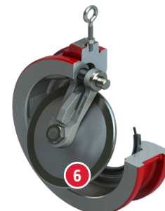
Figure 02: Seat Ring Soft Seat Cutaway Rear View.
