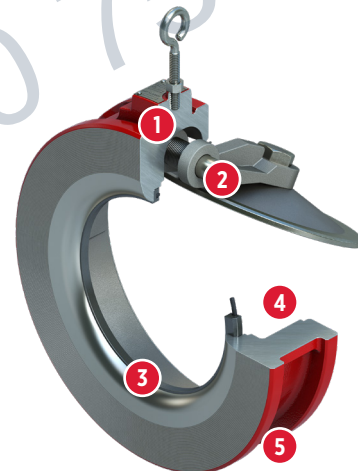
Figure 01: Seat Ring Soft Seat Cutaway Front View.
