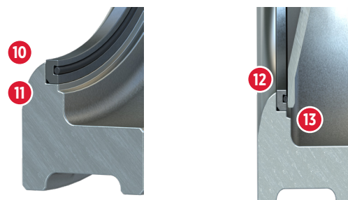
Figure 05: Seat Ring Soft Seat Close-Up Cutaway Views.
