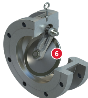
Figure 02: Integral Hard Seat Cutaway Rear View.
