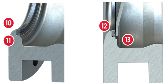
Figure 05: Seat Ring Soft Seat Close-Up Cutaway Views.
