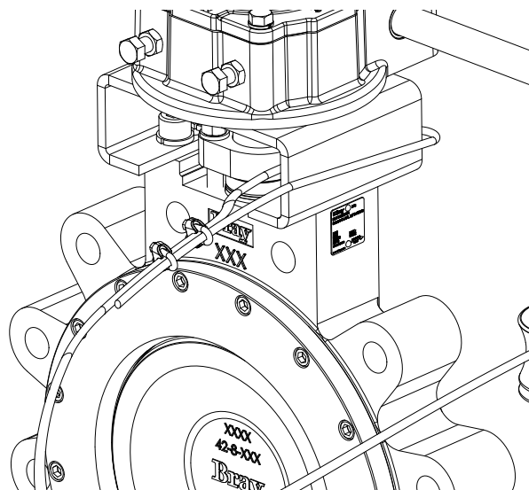
Figure 11 Wire cable secured around the bracket of the valve.
