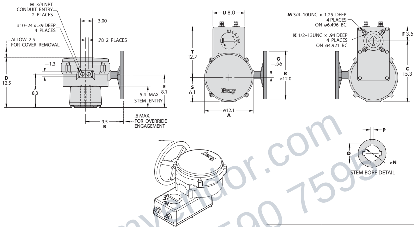
STEM BORE DETAIL
