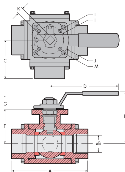
MPT/MPS/MPB - 230* - 1/4" - 2" shown
