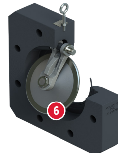
Figure 02: Integral Soft Seat Cutaway Rear View.
