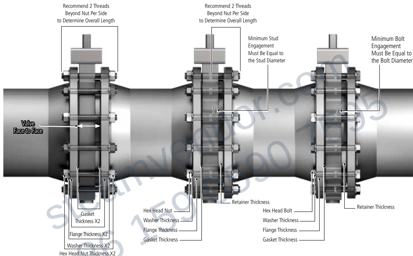
Wafer Valve
