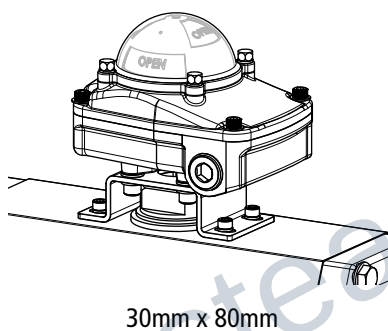
Single Piece Bracket
