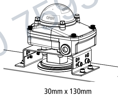
Adjustable Bracket for both 30x80 and 30x130 NAMUR mounting pads (fits all S92/93/98 actuators)
