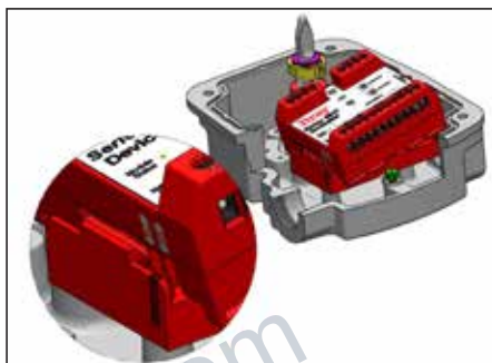
Figure 6: Pitching of the electronics package to begin installation
