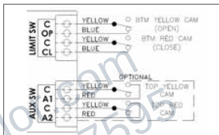
Figure 3: Factory wiring of the CommPro module
