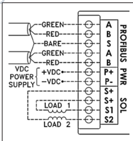
Figure 1: Field wiring of the CommPro
