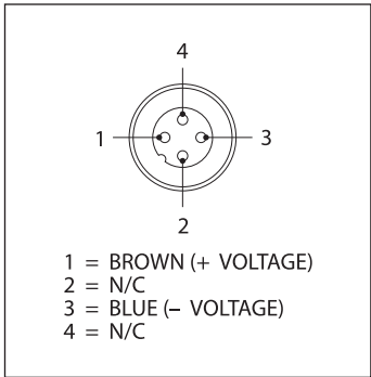
Figure 2: AS-i Male M12 Connector
