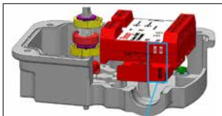
Figure 5: Alignment of appropriate slot
