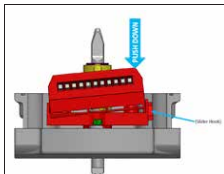
Figure 7: Push down on electronics package until the slider hook snaps in place
