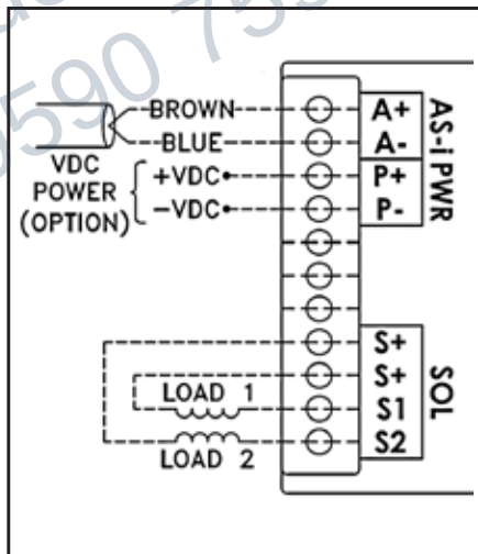
Figure 1: Field wiring of the CommPro
