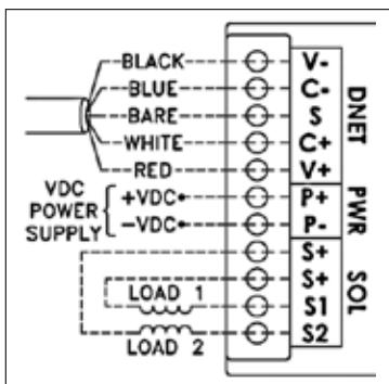
Figure 1: Field wiring of the CommPro
