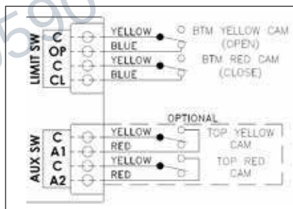
Figure 3: Factory wiring of the CommPro module
