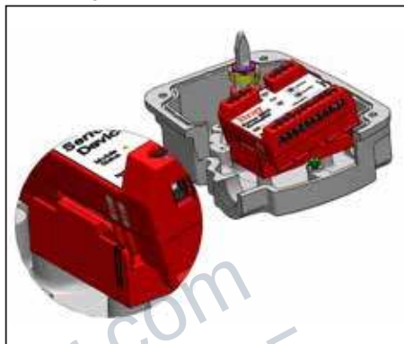
Figure 8: Pitching of the electronics package to begin installation
