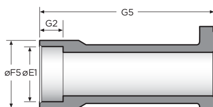
EXTENDED SOCKET WELD END 72E00/82E00
