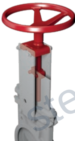
Non-Rising Stem
