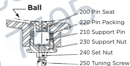
Ball Support
