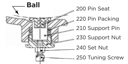
Figure 1 - Ball Support
