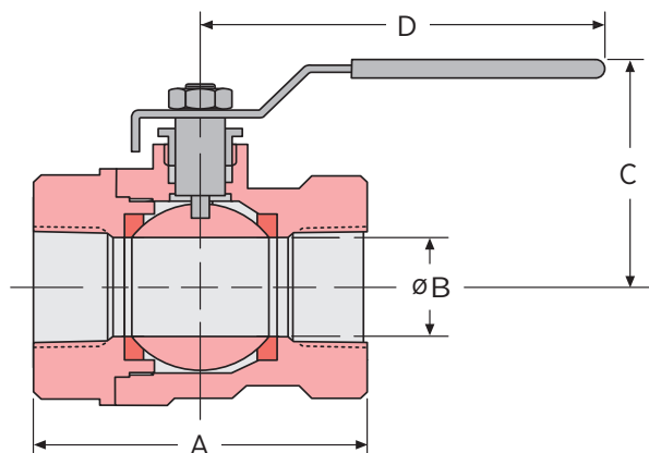
Dimensions (inch)
