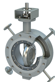
Steam Jackets
