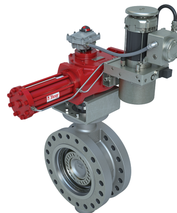
Tri Lok®-Cx shown with Series 98EH actuator with electro-hydraulic power pack.
