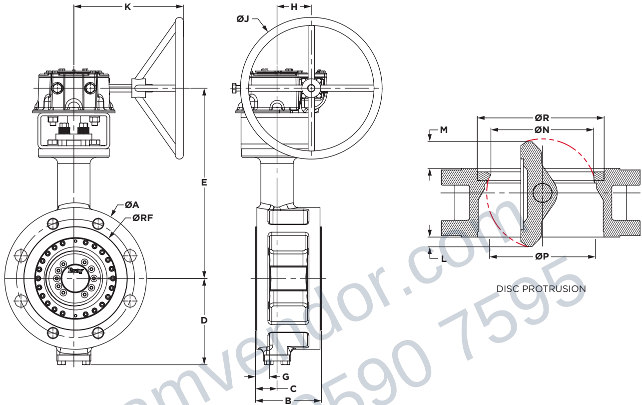
DIMENSIONS (mm)
