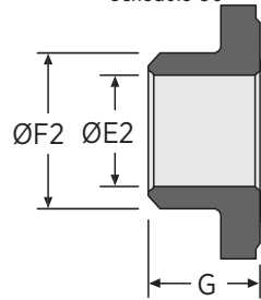
Butt Weld End Schedule 80
