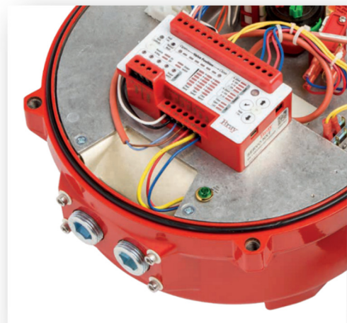
Bray's Servo Next module integrated with Servo Next for Control
