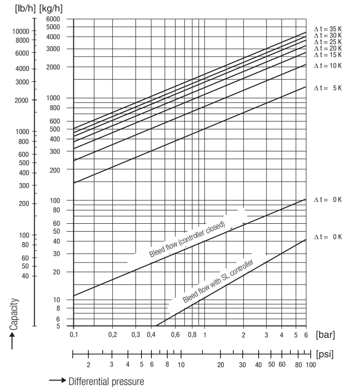
BW 31, DN 15 mm (½")
