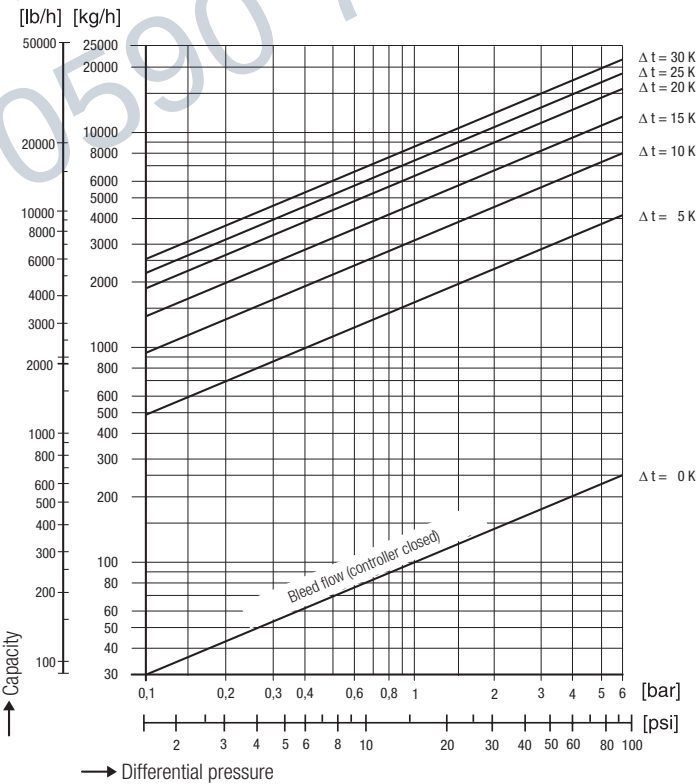
BW 31, DN 40 mm (1½")
