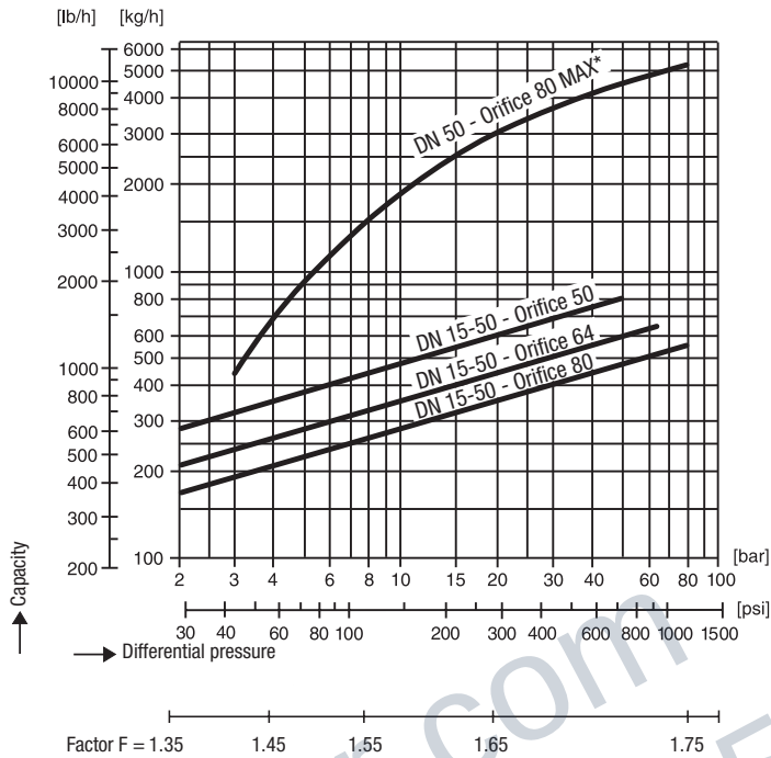
Additional cold-water start-up capacity due to thermostatic capsule DUPLEX design (only UNA 38)
