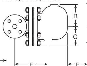
FT47 DN25, DN40和DN50
