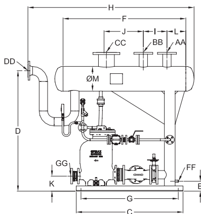
MFP14 DN25, DN40, DN50, DN80单泵组
