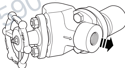
Fig. 2 USM21 fitted to a PC3_ pipeline connector
